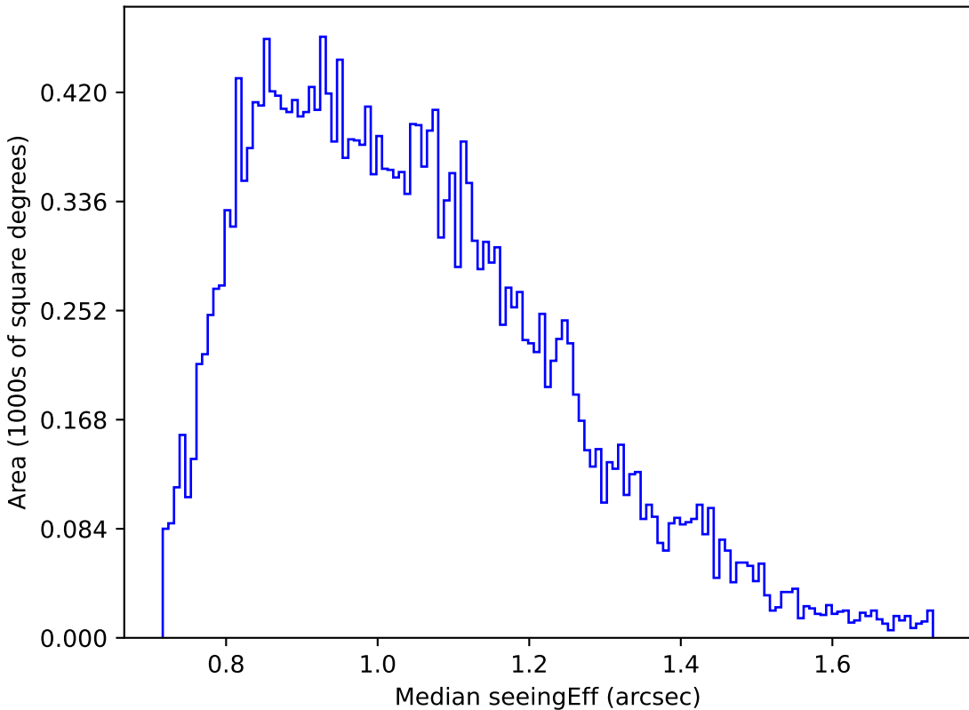
baseline_v3.2_10yrs Yr 1 g band: Median seeingEff
