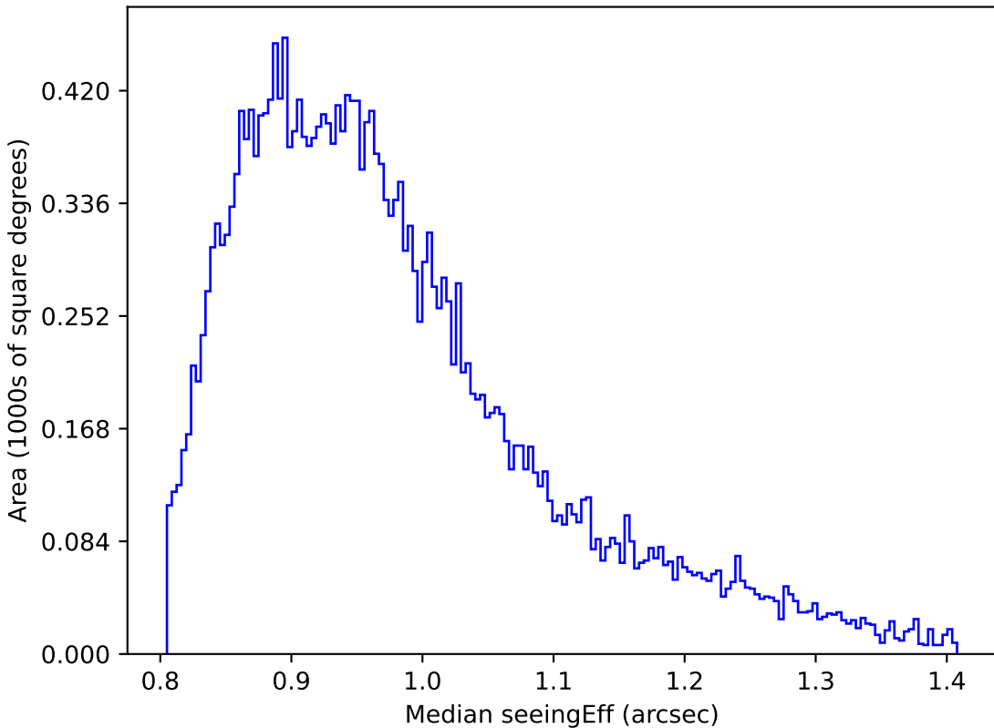
baseline_v3.2_10yrs Yr 1 all bands: Median seeingEff
