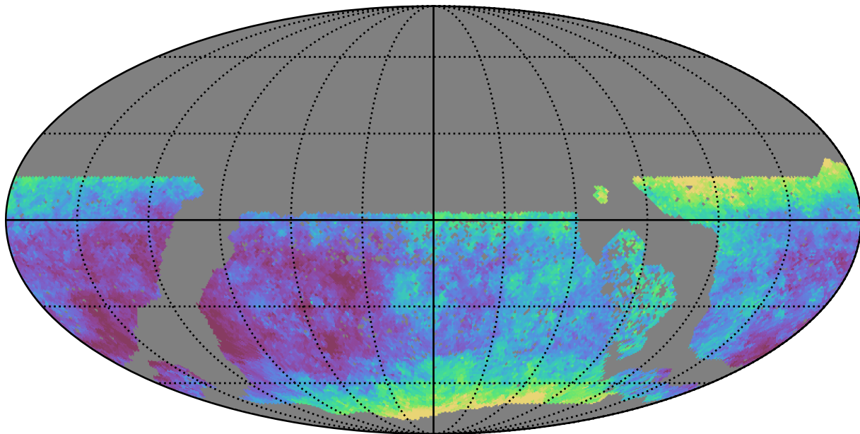
baseline_v3.2_10yrs WFD y band: Median seeingEff
