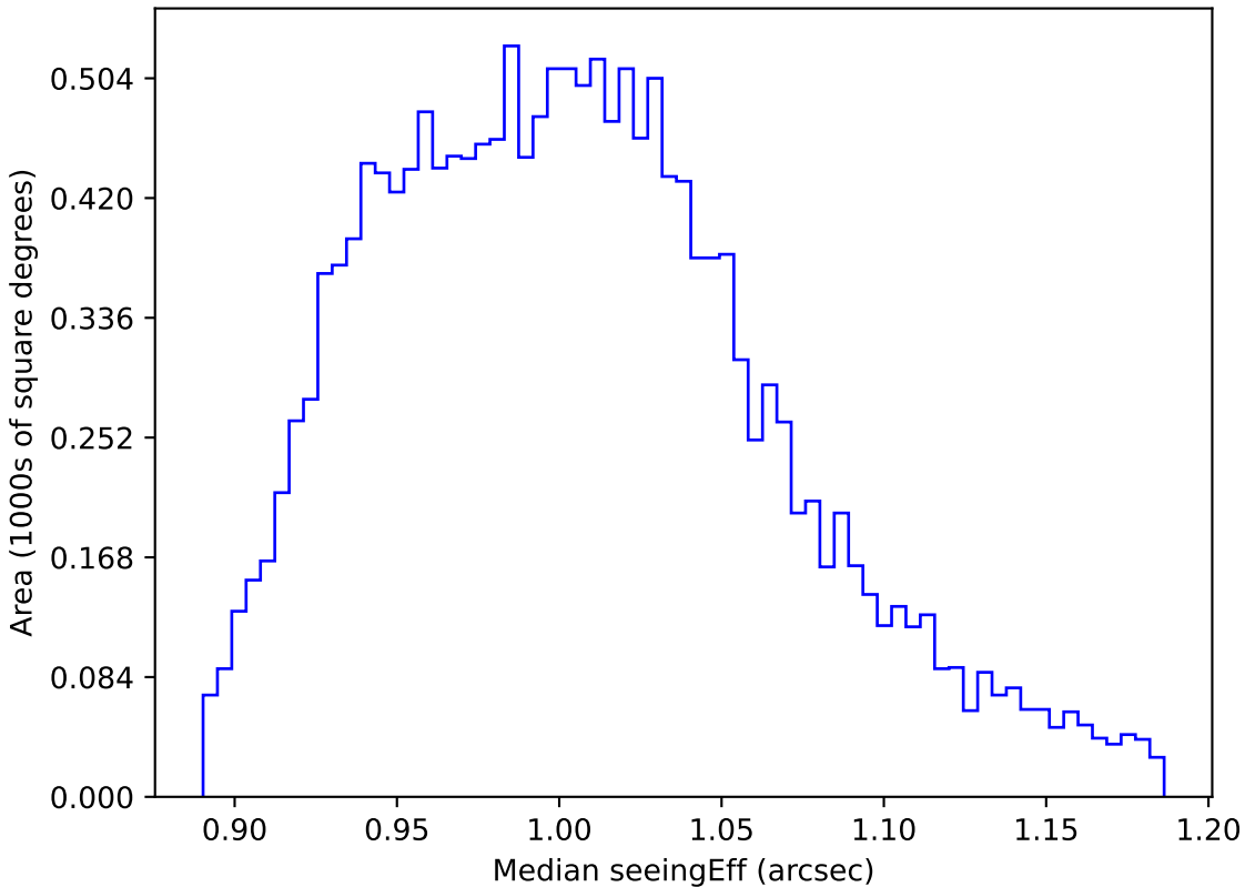
baseline_v3.2_10yrs WFD y band: Median seeingEff
