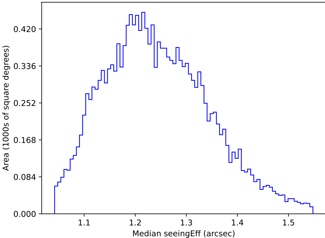
baseline_v3.2_10yrs WFD u band: Median seeingEff
