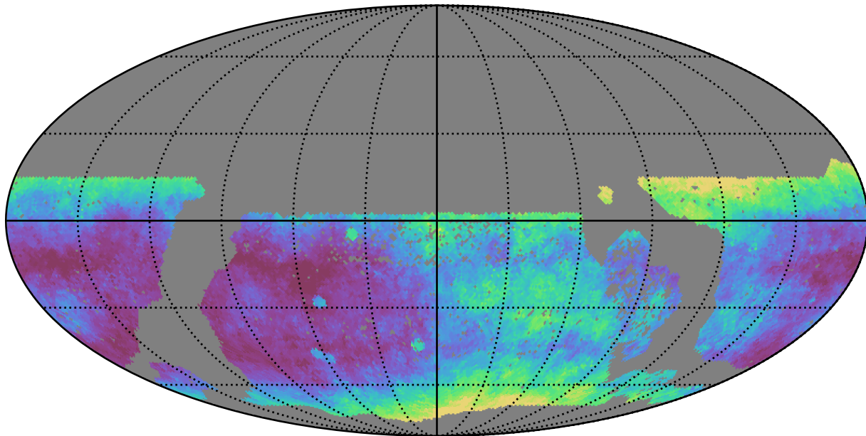
baseline_v3.2_10yrs WFD r band: Median seeingEff
