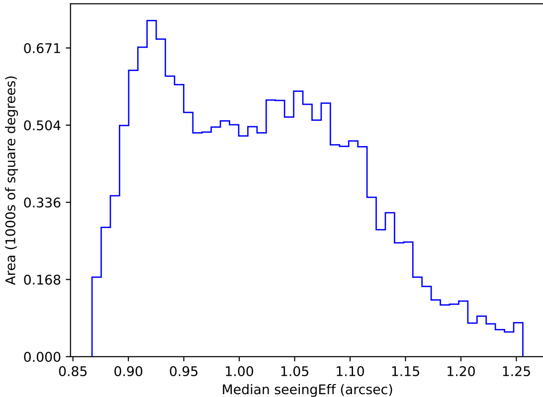
baseline_v3.2_10yrs WFD r band: Median seeingEff
