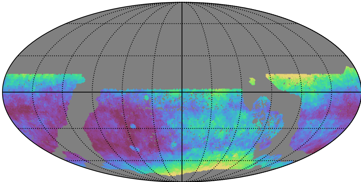
baseline_v3.2_10yrs WFD i band: Median seeingEff
