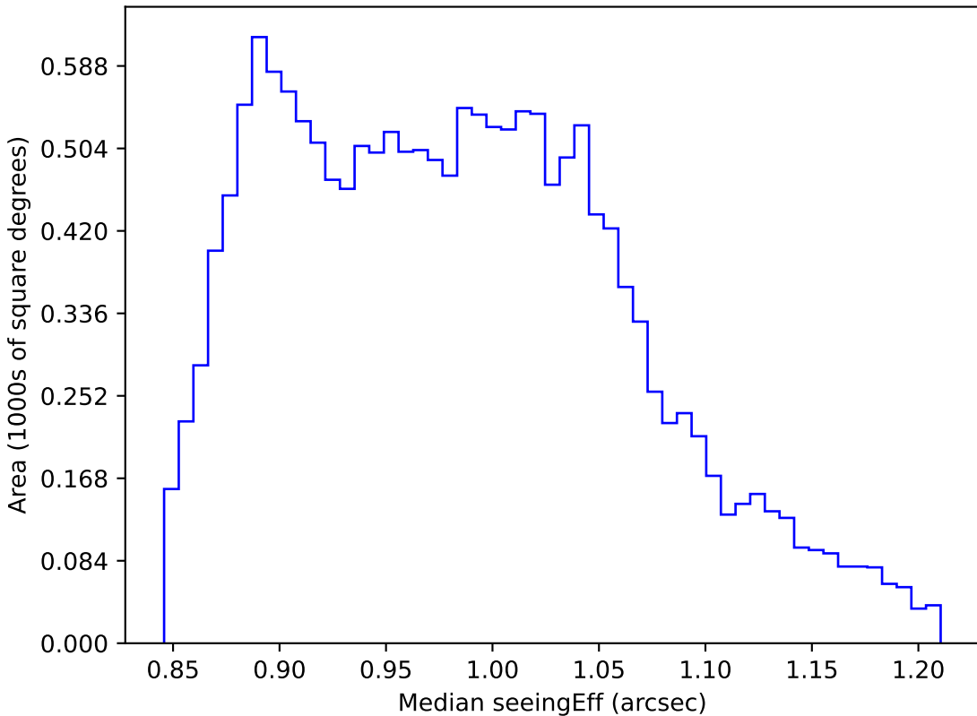
baseline_v3.2_10yrs WFD i band: Median seeingEff
