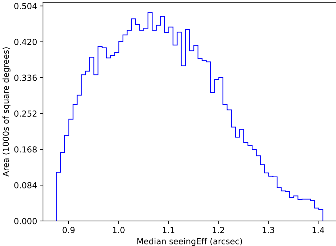
baseline_v3.2_10yrs WFD g band: Median seeingEff
