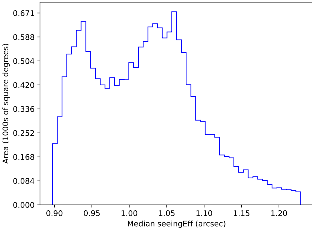
baseline_v3.2_10yrs WFD all bands: Median seeingEff
