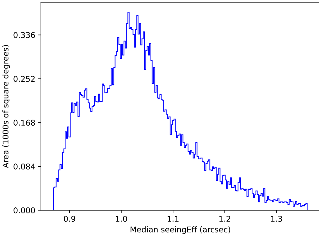
baseline_v3.2_10yrs All sky z band: Median seeingEff
