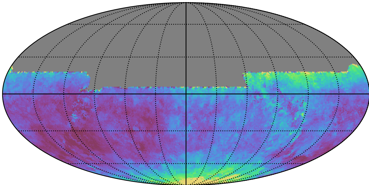
baseline_v3.2_10yrs All sky y band: Median seeingEff
