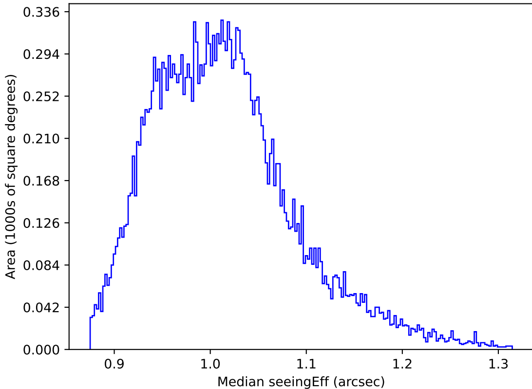
baseline_v3.2_10yrs All sky y band: Median seeingEff
