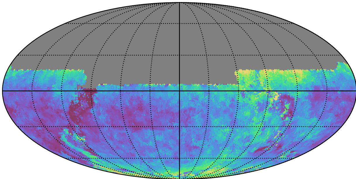
baseline_v3.2_10yrs All sky u band: Median seeingEff
