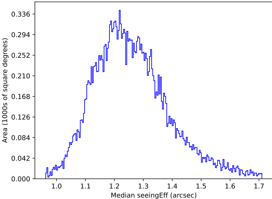
baseline_v3.2_10yrs All sky u band: Median seeingEff
