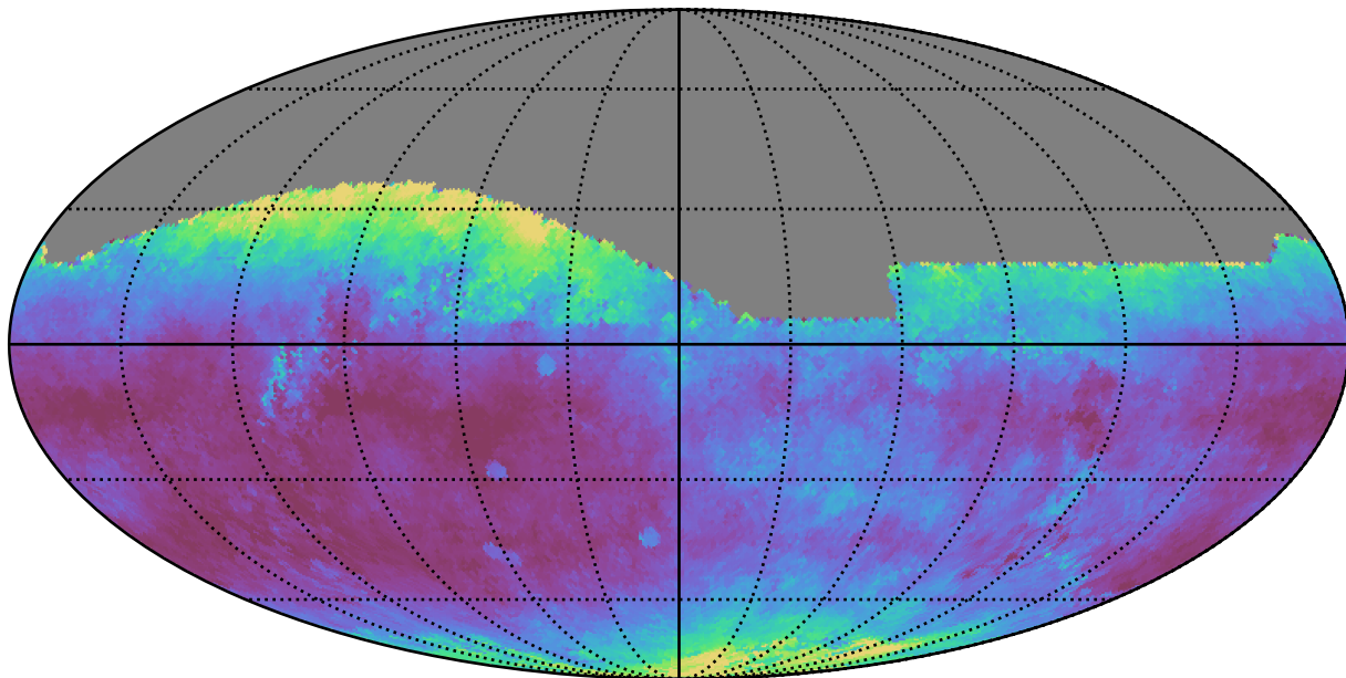
baseline_v3.2_10yrs All sky r band: Median seeingEff
