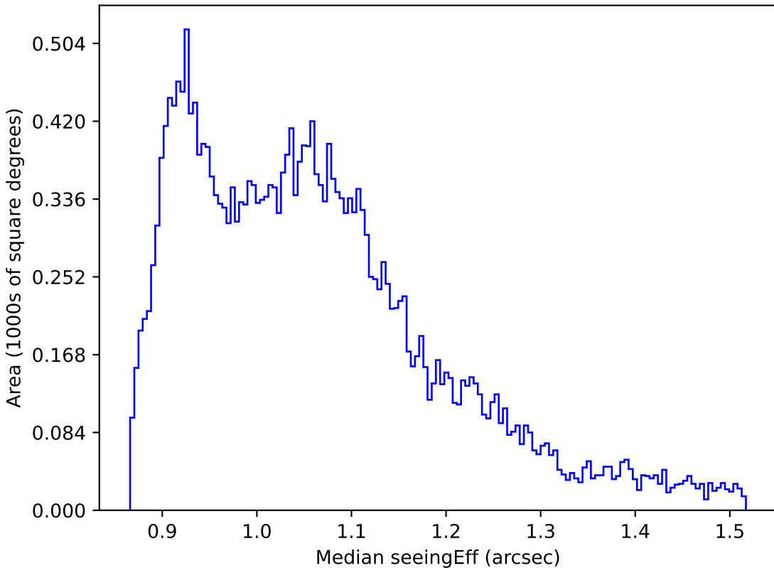
baseline_v3.2_10yrs All sky r band: Median seeingEff
