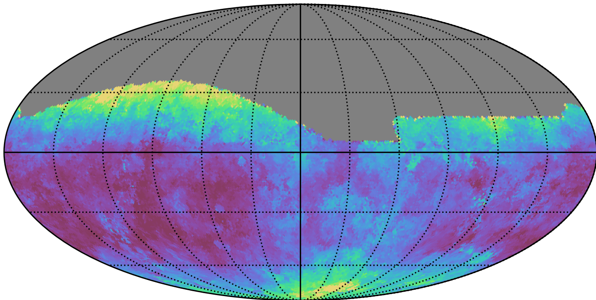
baseline_v3.2_10yrs All sky g band: Median seeingEff
