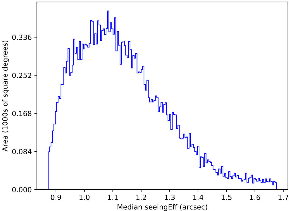
baseline_v3.2_10yrs All sky g band: Median seeingEff
