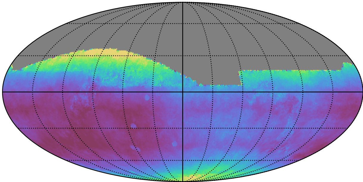
baseline_v3.2_10yrs All sky all bands: Median seeingEff
