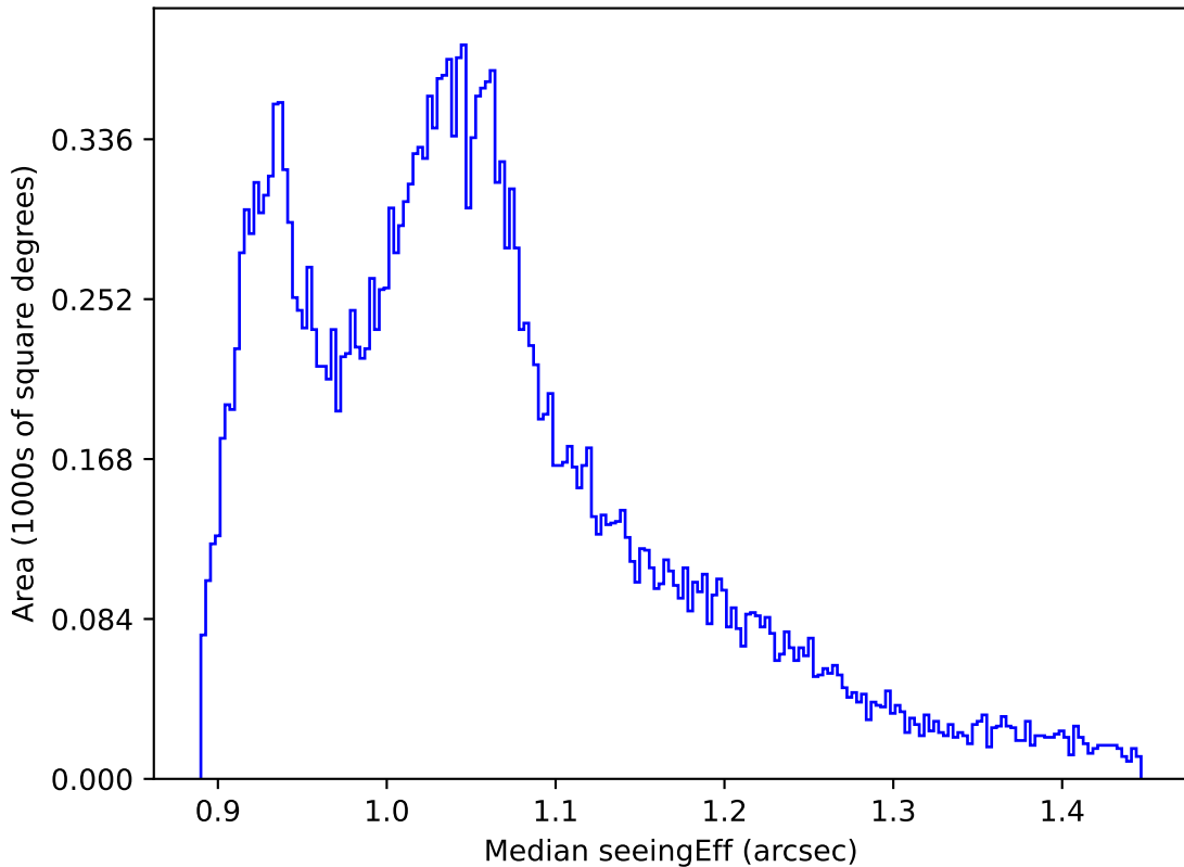
baseline_v3.2_10yrs All sky all bands: Median seeingEff
