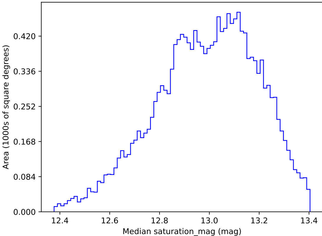
baseline_v3.2_10yrs WFD u band: Median saturation_mag
