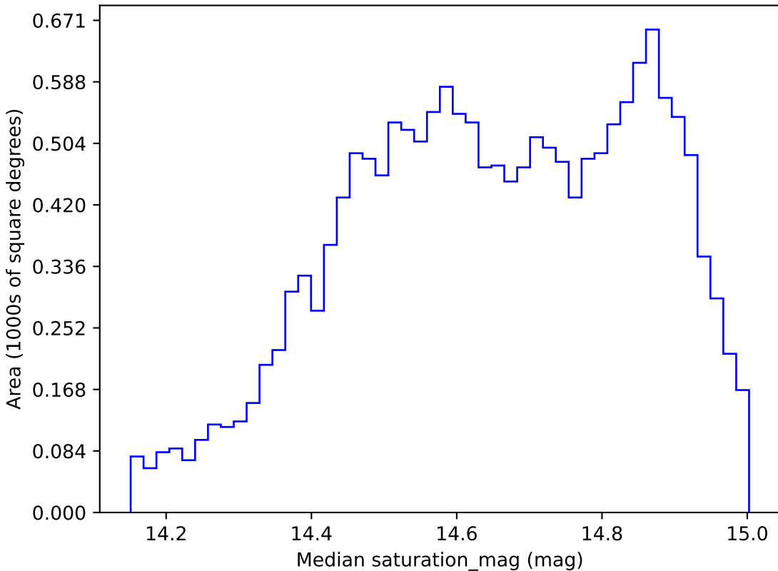
baseline_v3.2_10yrs WFD r band: Median saturation_mag
