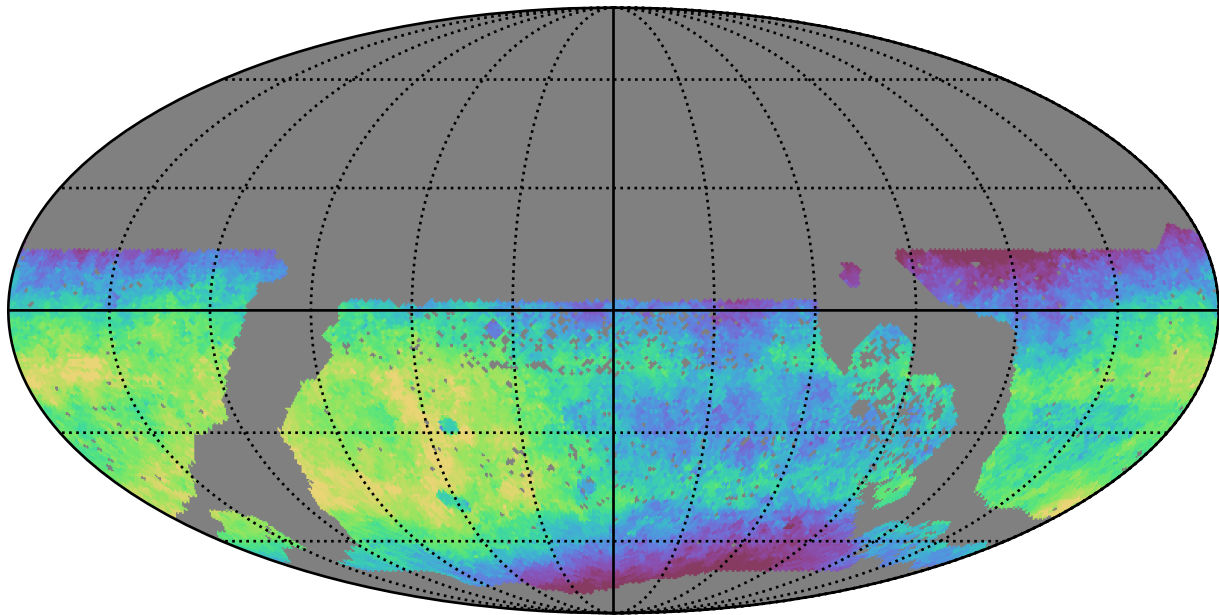
baseline_v3.2_10yrs WFD i band: Median saturation_mag
