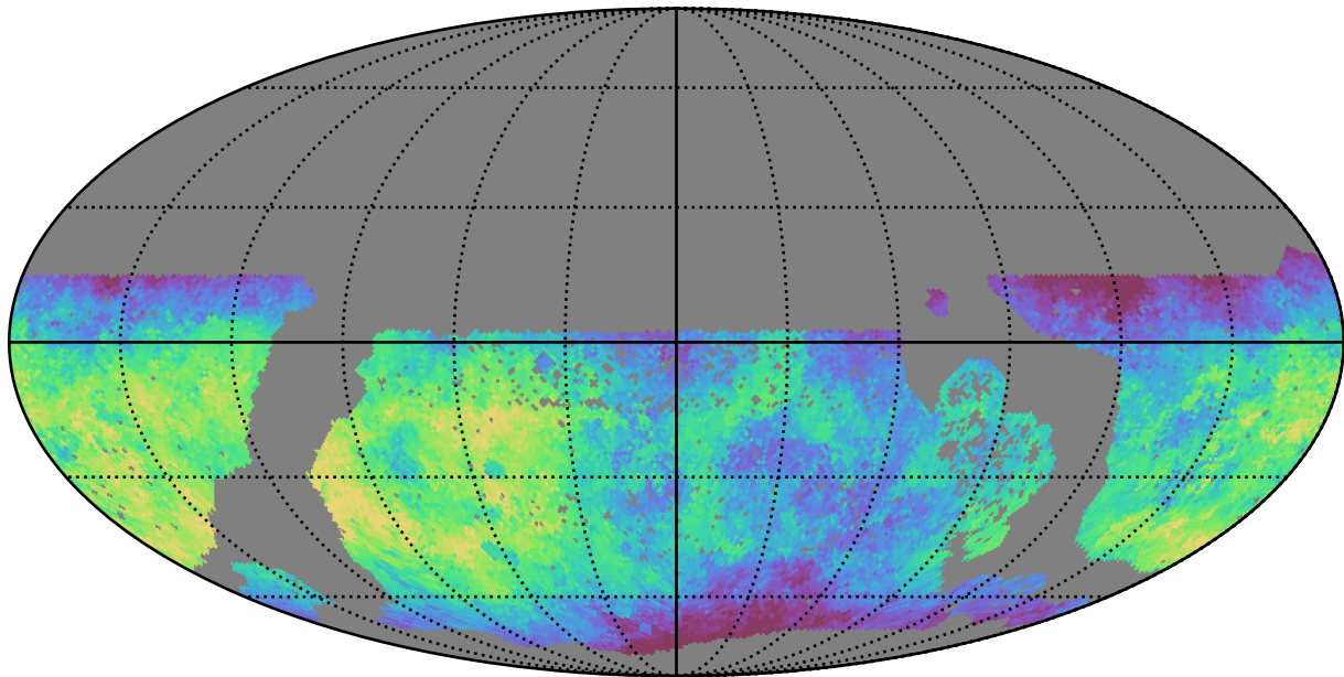
baseline_v3.2_10yrs WFD g band: Median saturation_mag
