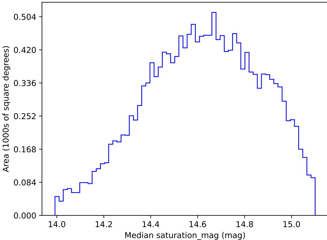
baseline_v3.2_10yrs WFD g band: Median saturation_mag
