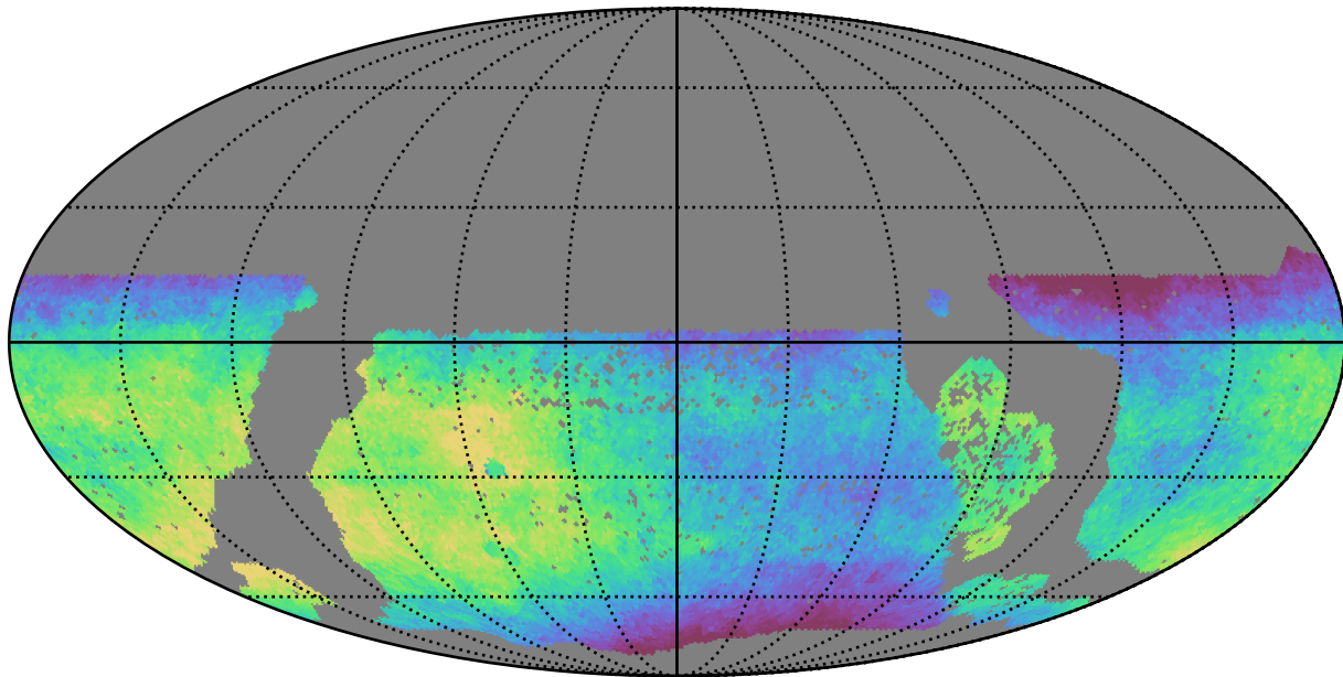
baseline_v3.2_10yrs WFD all bands: Median saturation_mag
