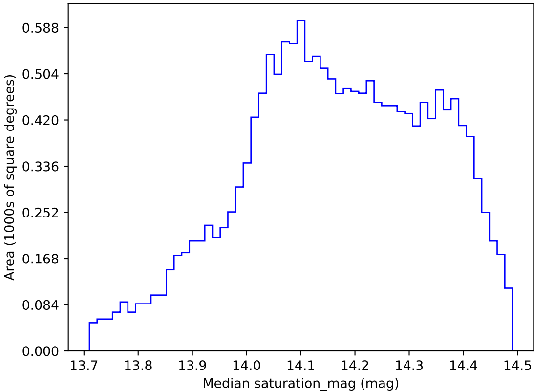
baseline_v3.2_10yrs WFD all bands: Median saturation_mag
