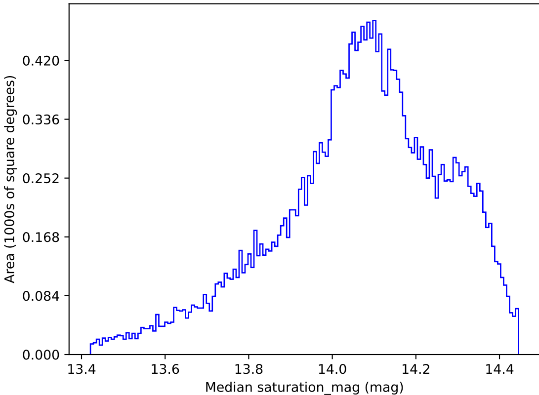
baseline_v3.2_10yrs All sky z band: Median saturation_mag
