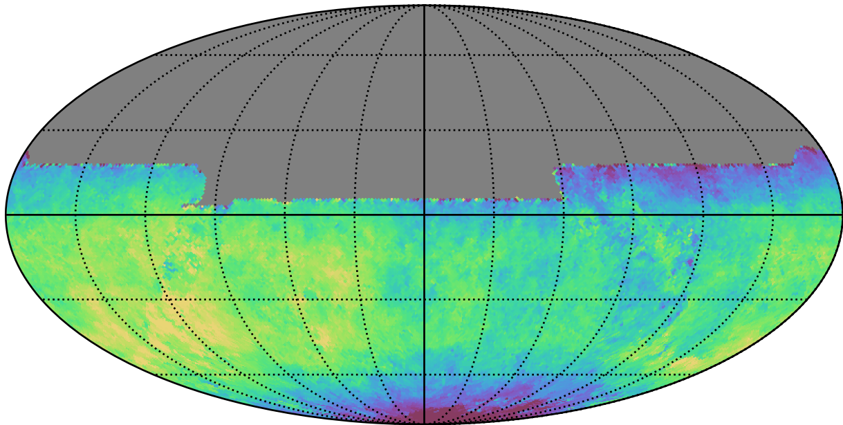
baseline_v3.2_10yrs All sky y band: Median saturation_mag
