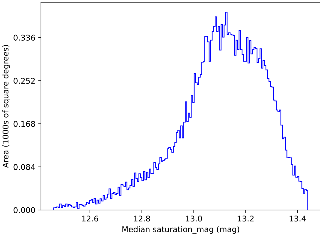
baseline_v3.2_10yrs All sky y band: Median saturation_mag
