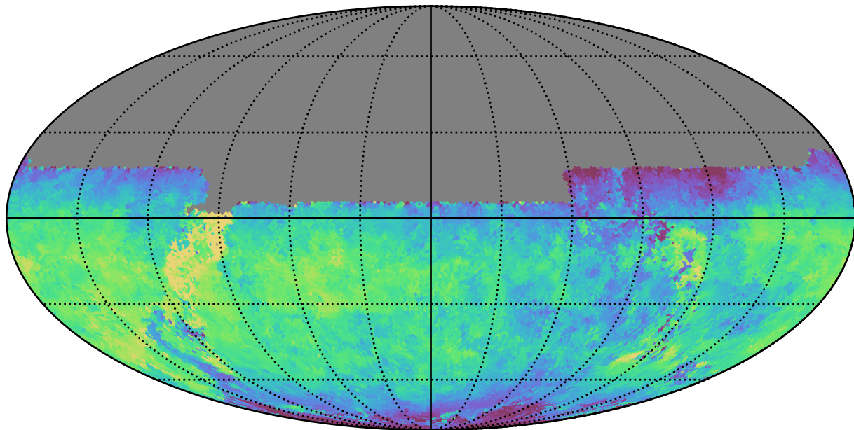
baseline_v3.2_10yrs All sky u band: Median saturation_mag
