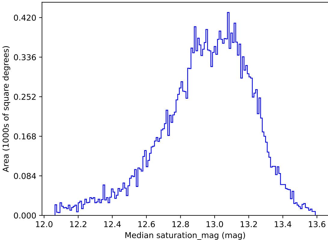
baseline_v3.2_10yrs All sky u band: Median saturation_mag
