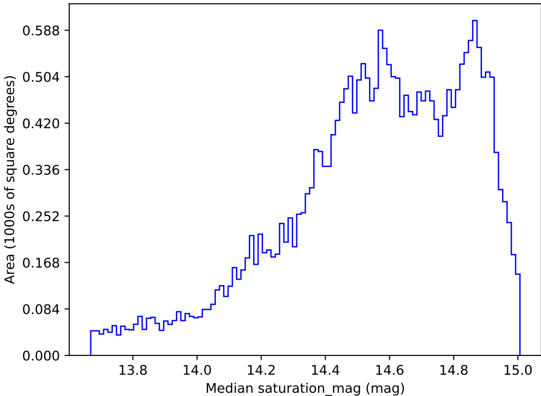
baseline_v3.2_10yrs All sky r band: Median saturation_mag
