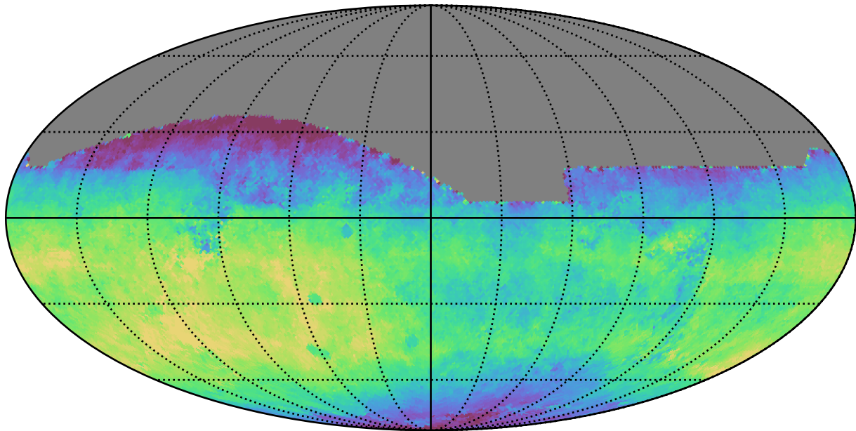
baseline_v3.2_10yrs All sky i band: Median saturation_mag
