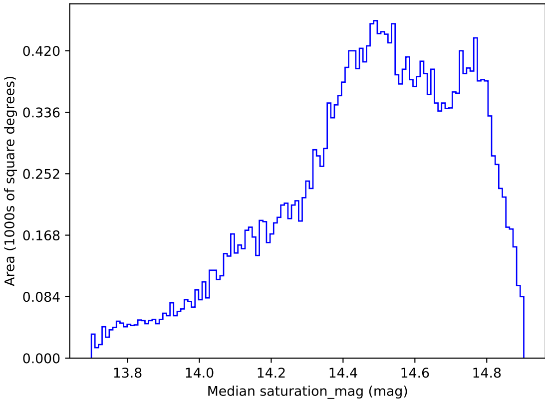
baseline_v3.2_10yrs All sky i band: Median saturation_mag
