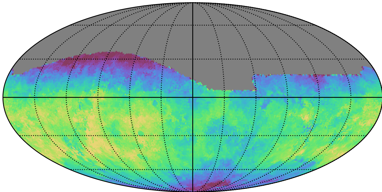
baseline_v3.2_10yrs All sky g band: Median saturation_mag
