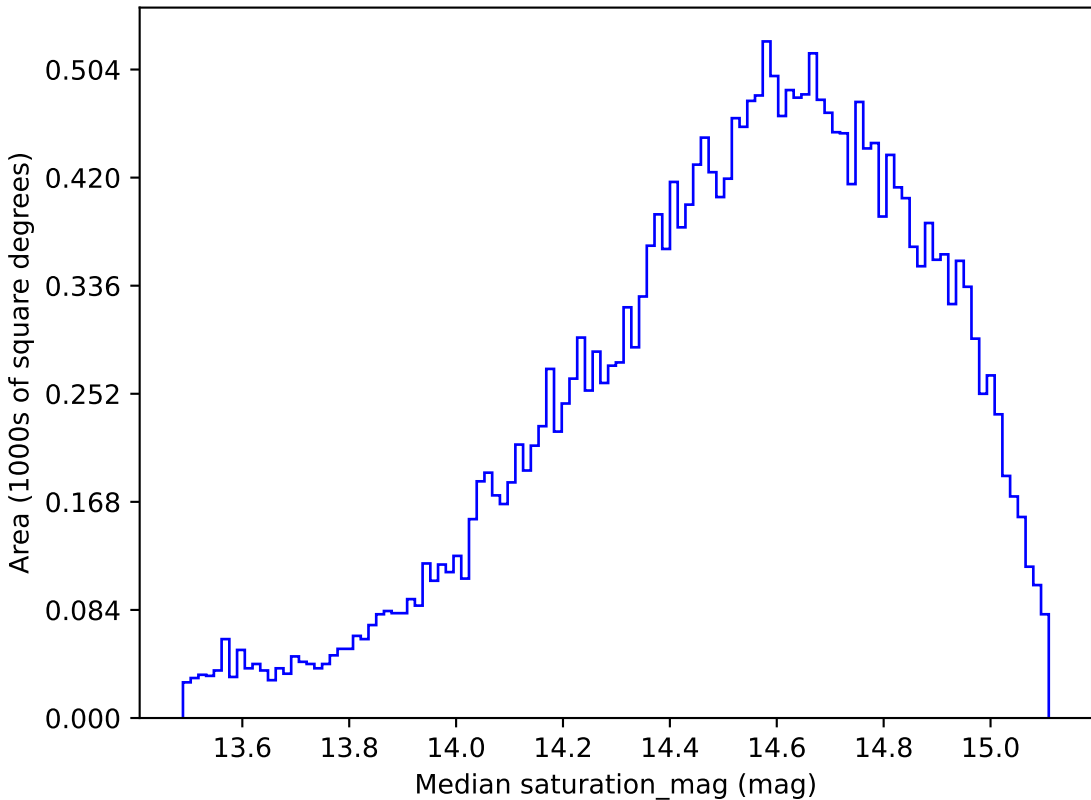
baseline_v3.2_10yrs All sky g band: Median saturation_mag
