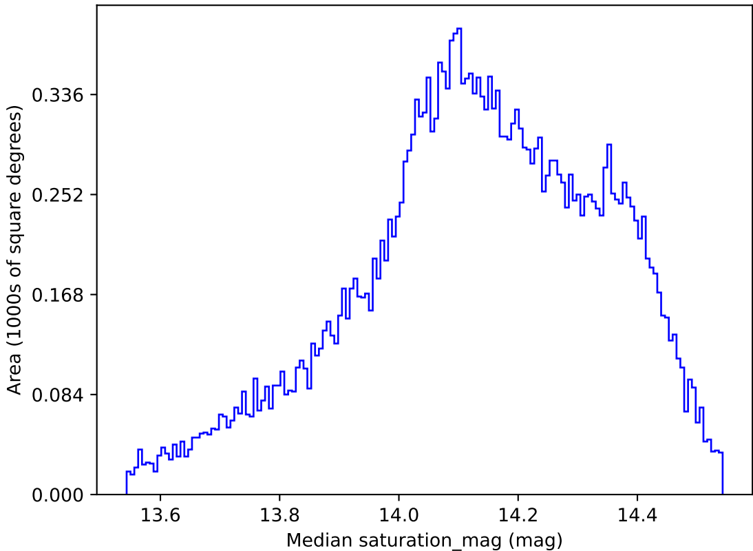
baseline_v3.2_10yrs All sky all bands: Median saturation_mag
