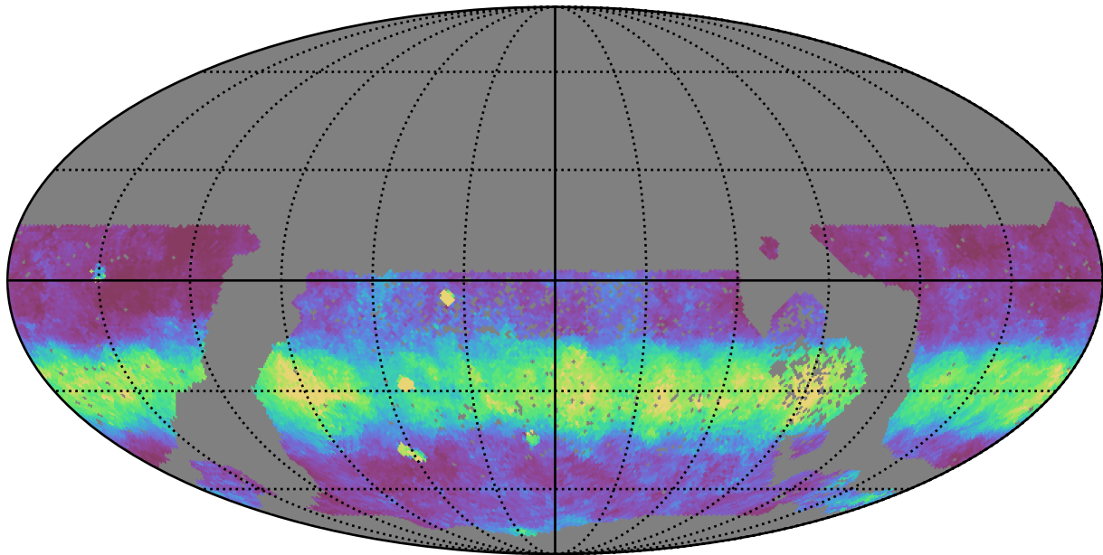
baseline_v3.2_10yrs WFD z band: Median normairmass
