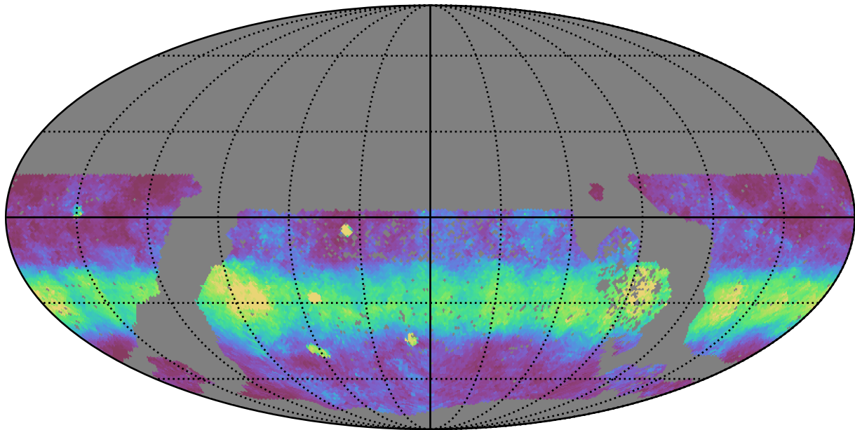
baseline_v3.2_10yrs WFD y band: Median normairmass
