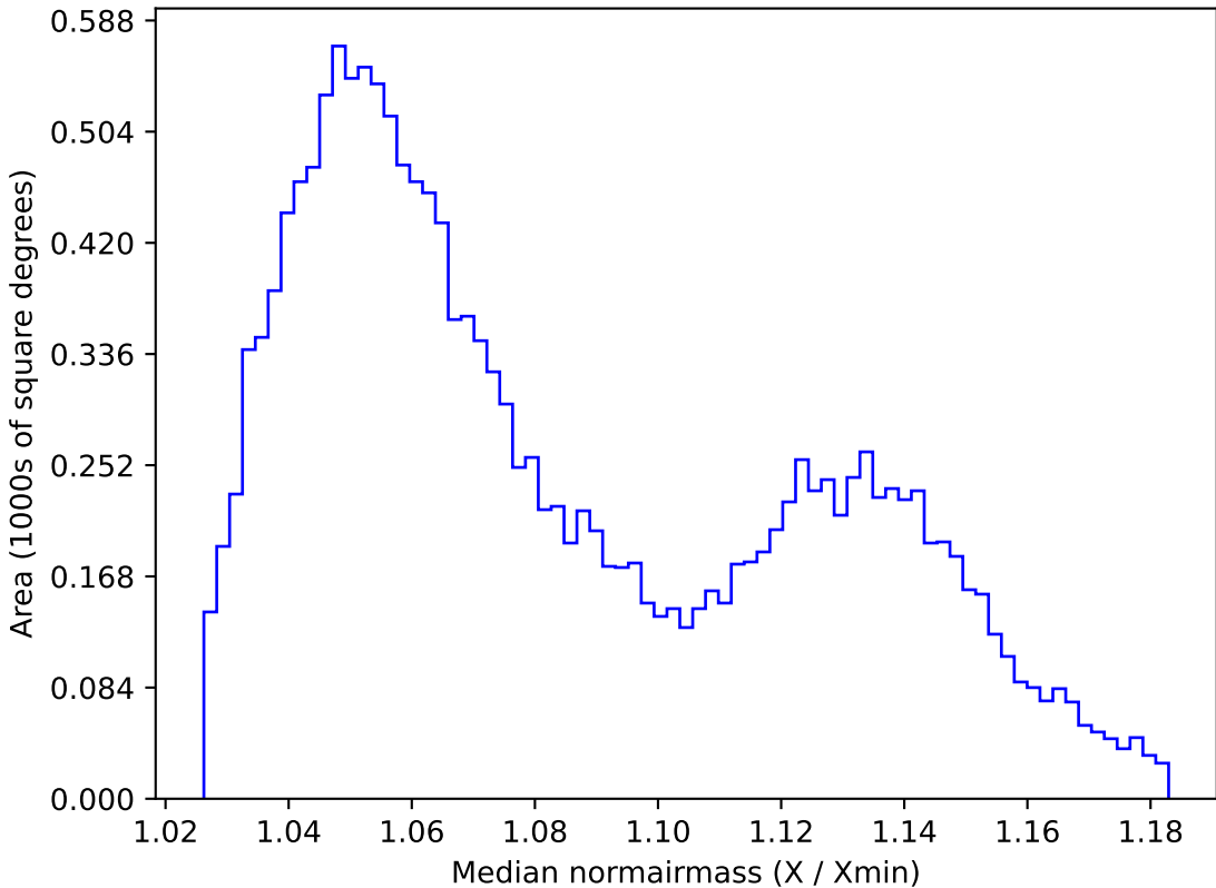
baseline_v3.2_10yrs WFD y band: Median normairmass
