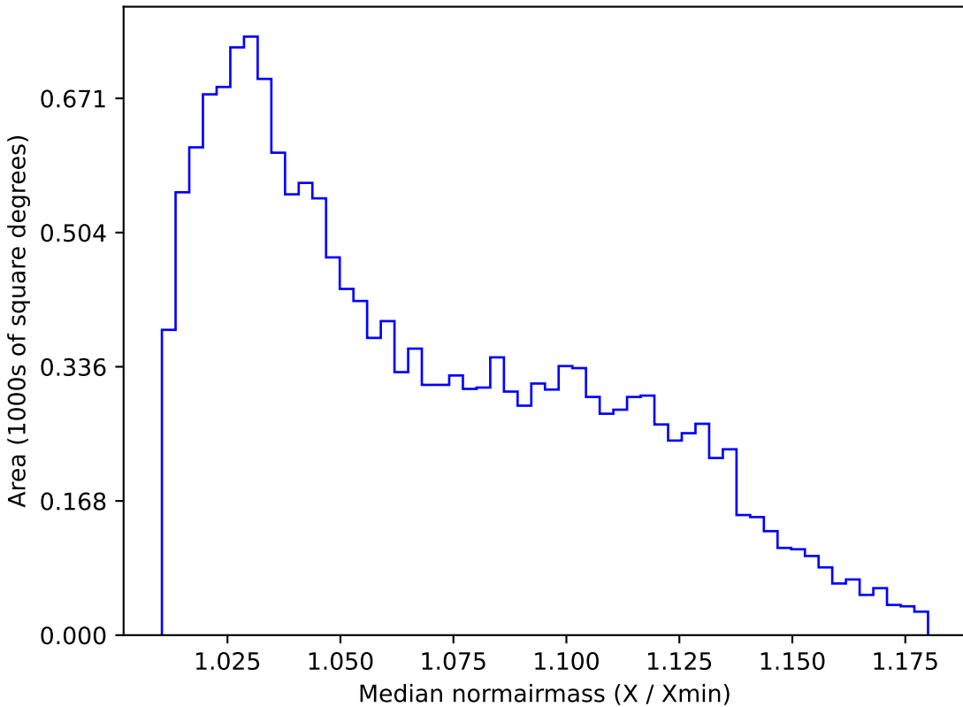
baseline_v3.2_10yrs WFD u band: Median normairmass
