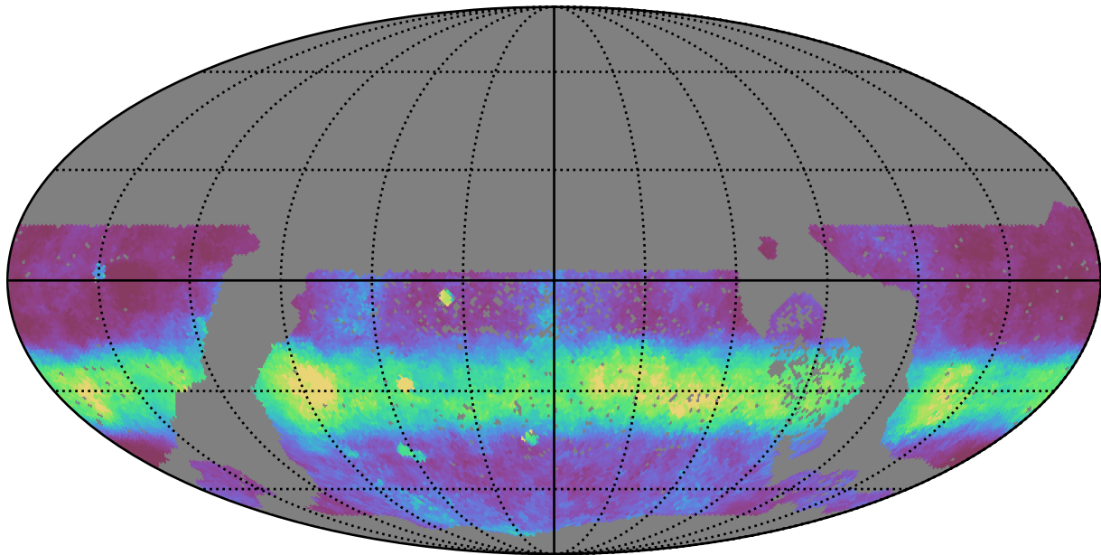
baseline_v3.2_10yrs WFD r band: Median normairmass
