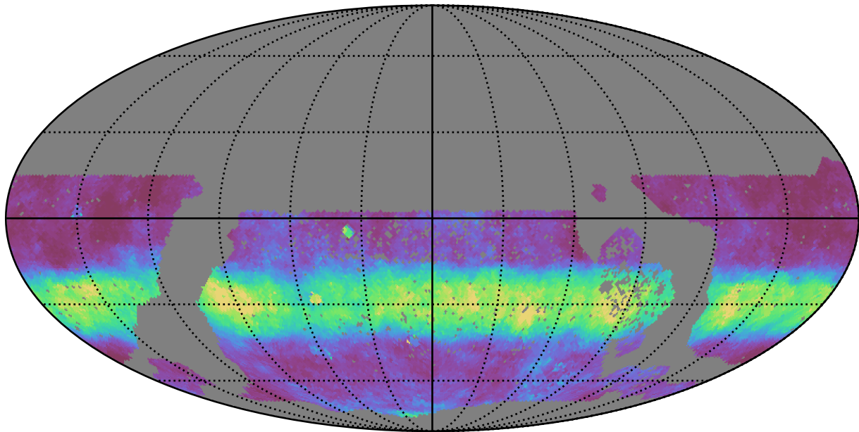
baseline_v3.2_10yrs WFD i band: Median normairmass
