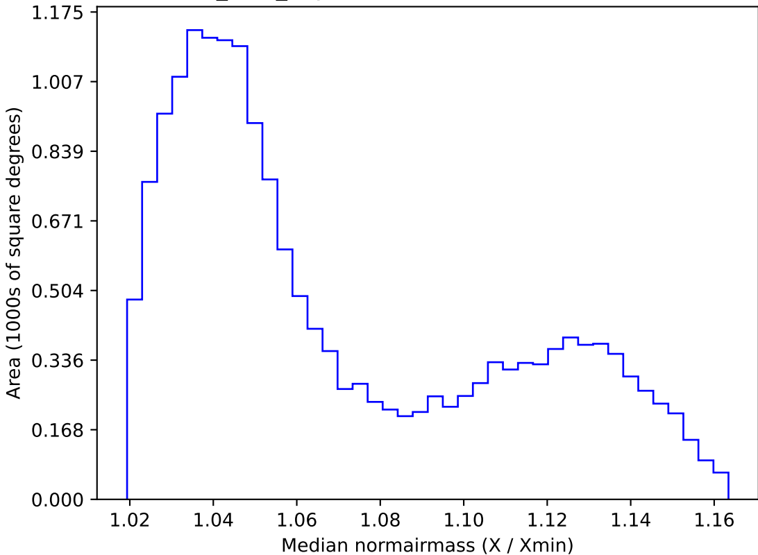
baseline_v3.2_10yrs WFD i band: Median normairmass
