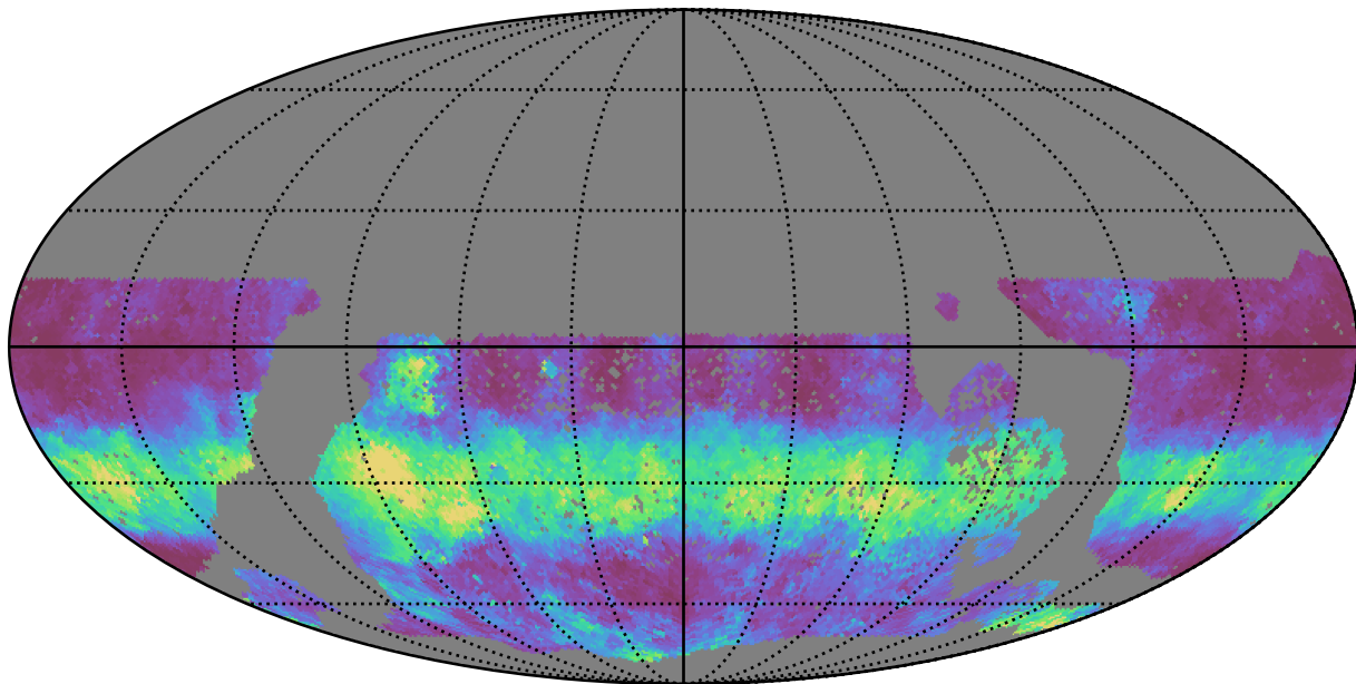
baseline_v3.2_10yrs WFD g band: Median normairmass
