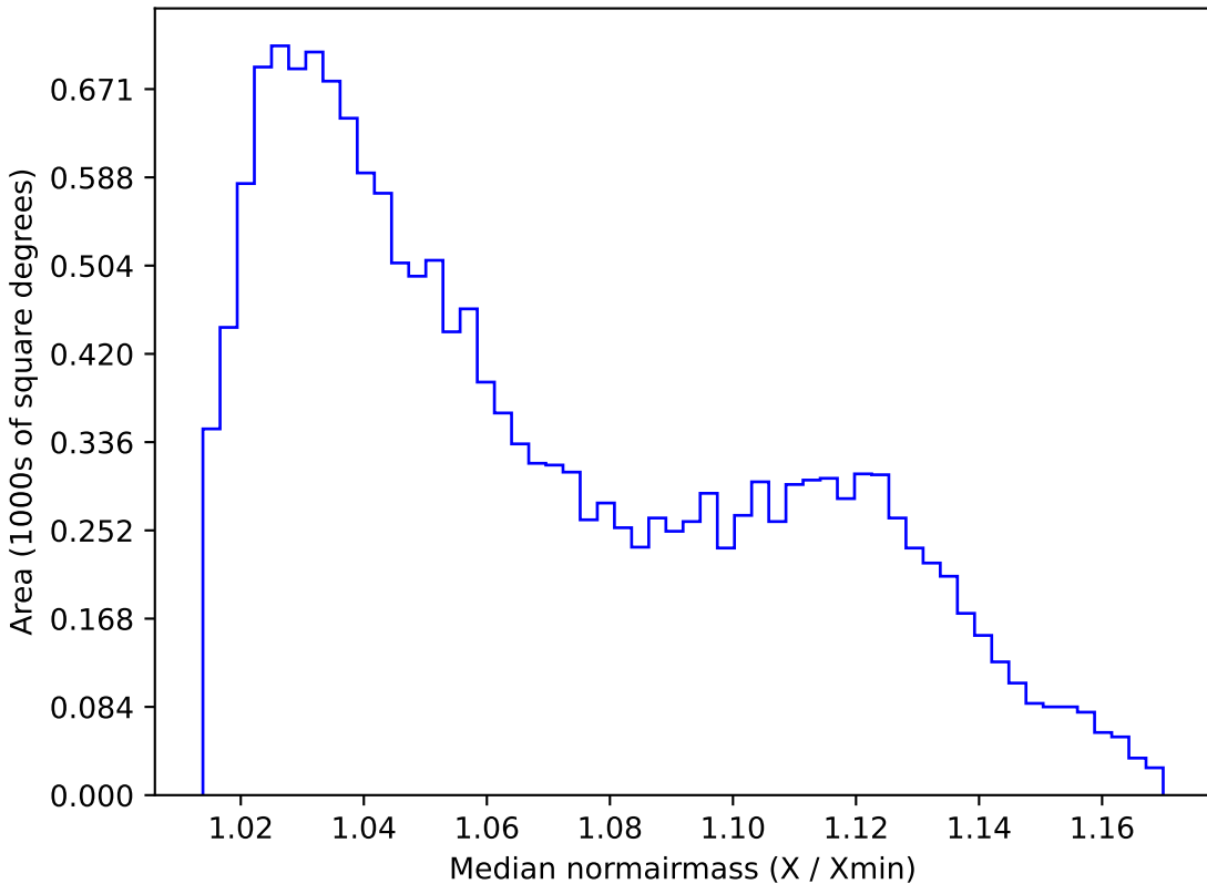
baseline_v3.2_10yrs WFD g band: Median normairmass
