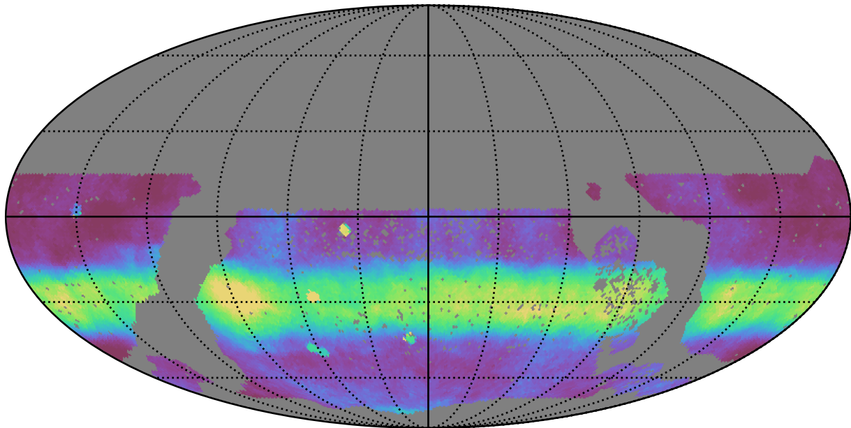
baseline_v3.2_10yrs WFD all bands: Median normairmass
